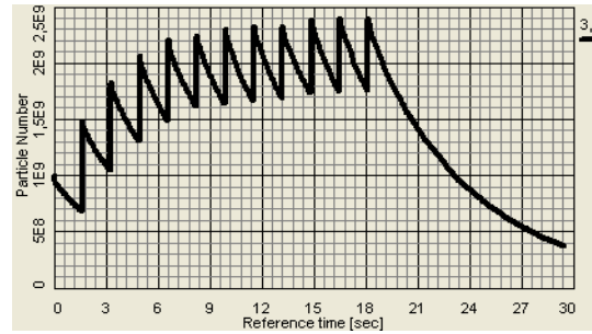
Fig.5 Dependence of the simulated stack intensity on time at HIMAC for I=100 mA and R=2.
