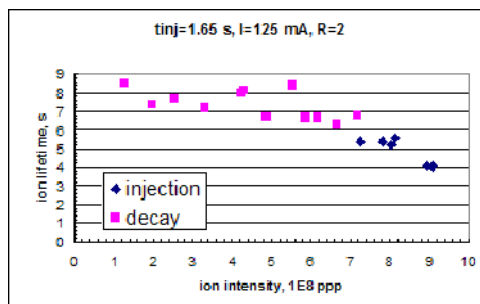
Fig.1 Ion lifetime versus ion intensity [1].
